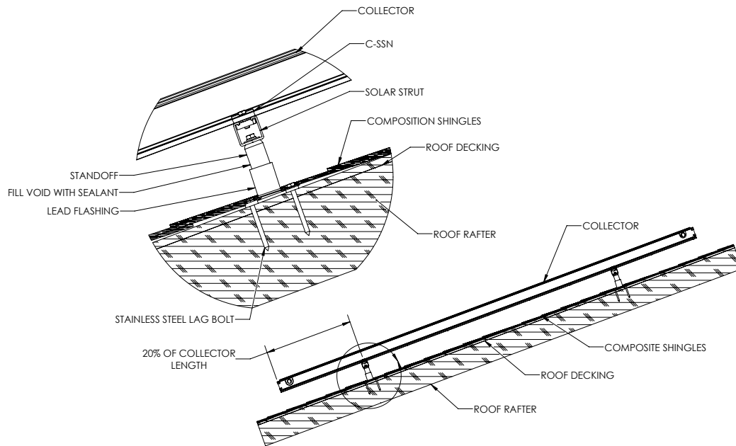
STRUT ON STANDOFF FOR COMPOSITION SHINGLE ROOF
