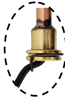
Wire-Clip holds the wire in place
